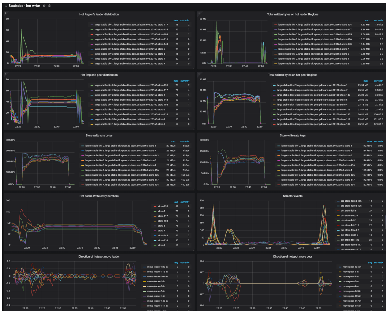
图 56: PD Dashboard - Hot write metrics
