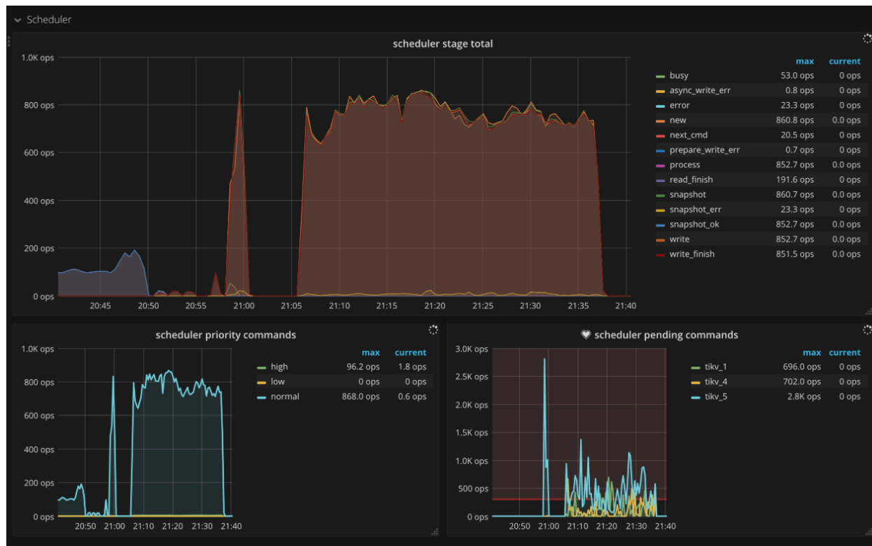
图 74: TiKV Dashboard - Scheduler metrics
