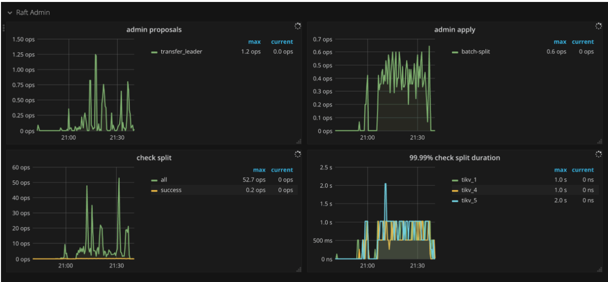
图 71: TiKV Dashboard - Raft admin metrics
