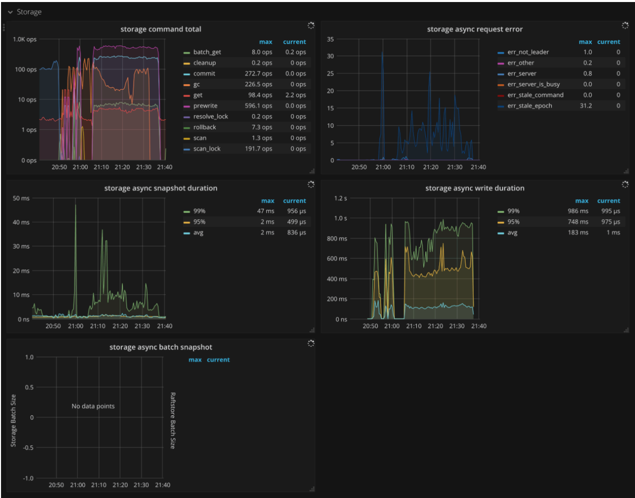
图 73: TiKV Dashboard - Storage metrics
