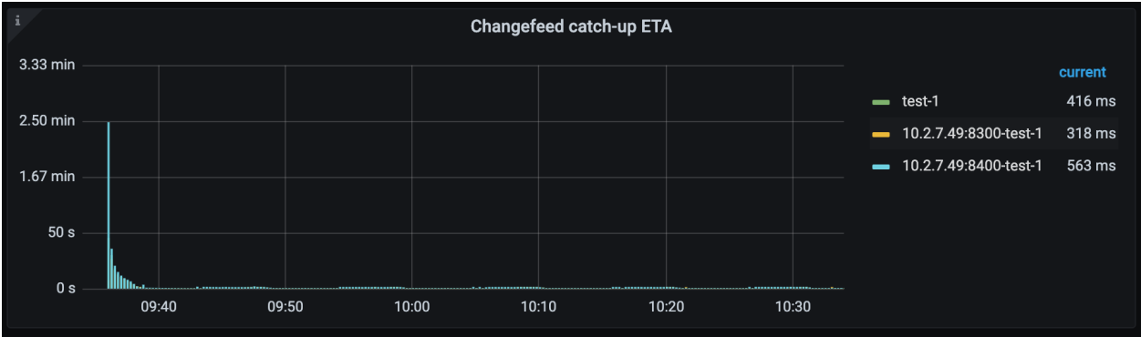
图 81: TiCDC Dashboard - Changefeed metrics 4
