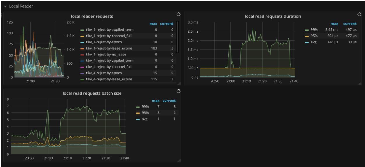
图 72: TiKV Dashboard - Local reader metrics
