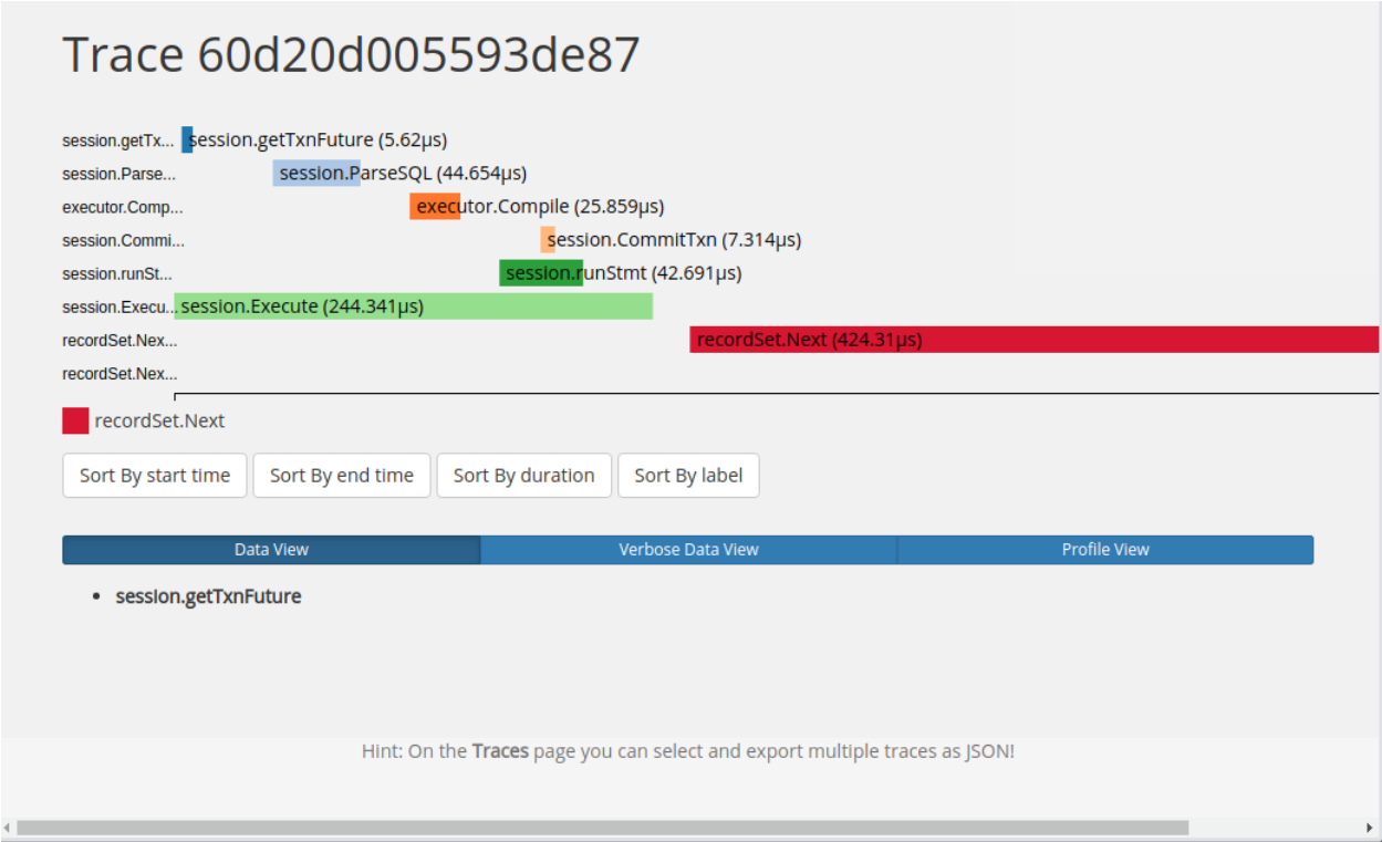
图 200: Trace Viewer-2
