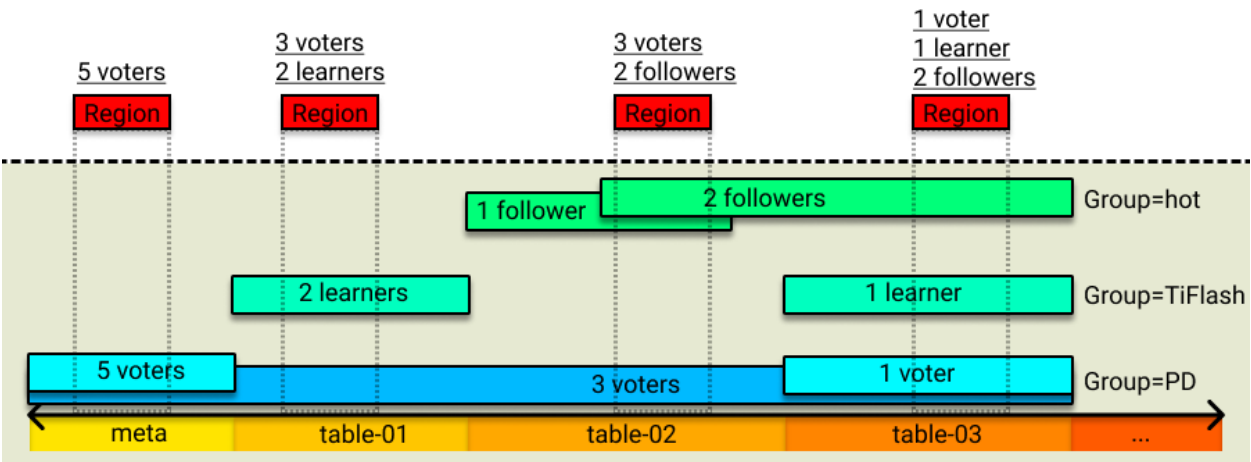
图 48: Placement rules overview
