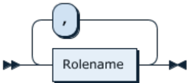
图 146: RolenameList
