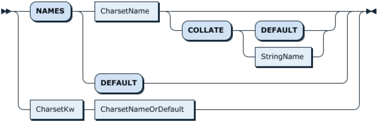
图 102: VariableAssignment
