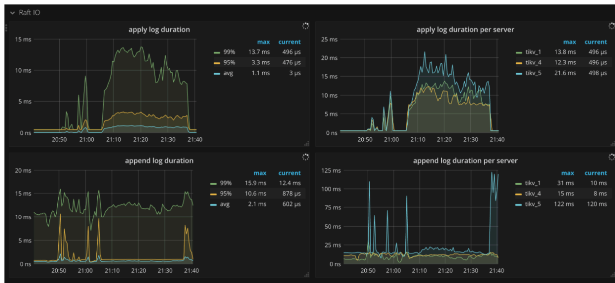
图 67: TiKV Dashboard - Raft IO metrics
