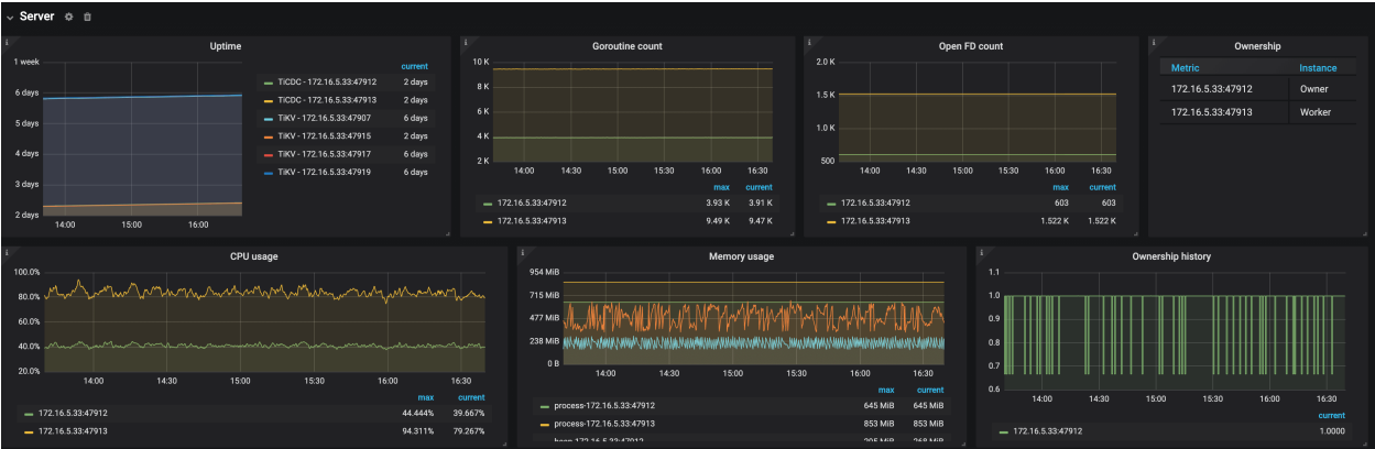
图 77: TiCDC Dashboard - Server metrics
