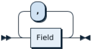
图 87: SelectStmtFieldList
