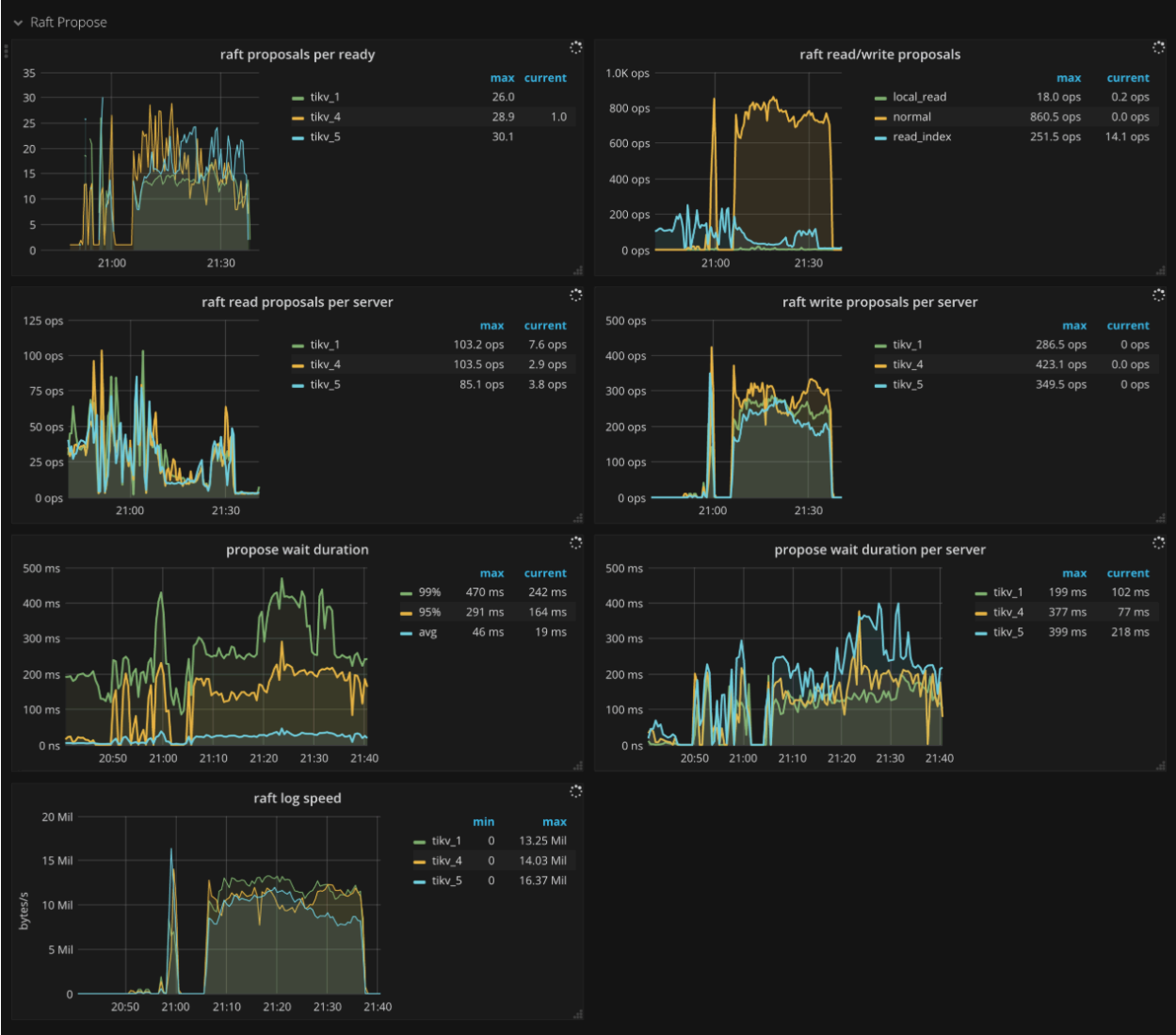
图 70: TiKV Dashboard - Raft propose metrics
