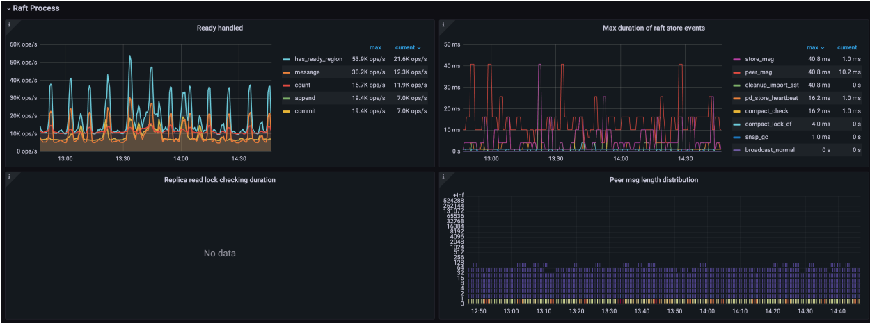
图 68: TiKV Dashboard - Raft process metrics
