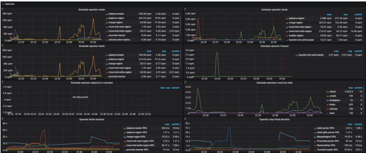
图 54: PD Dashboard - Operator metrics
